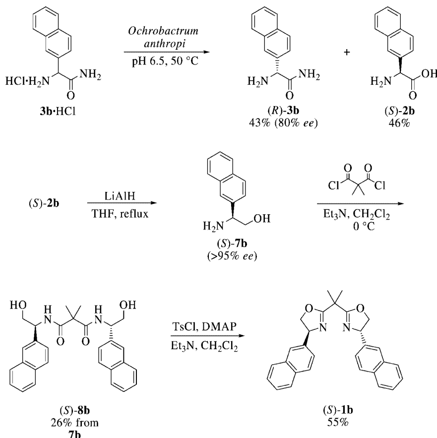
Scheme 3. Synthesis of ( S )-(2-naphthyl)bisoaxazoline ( 1b ).
